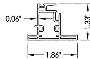
5 MEETING STILE
