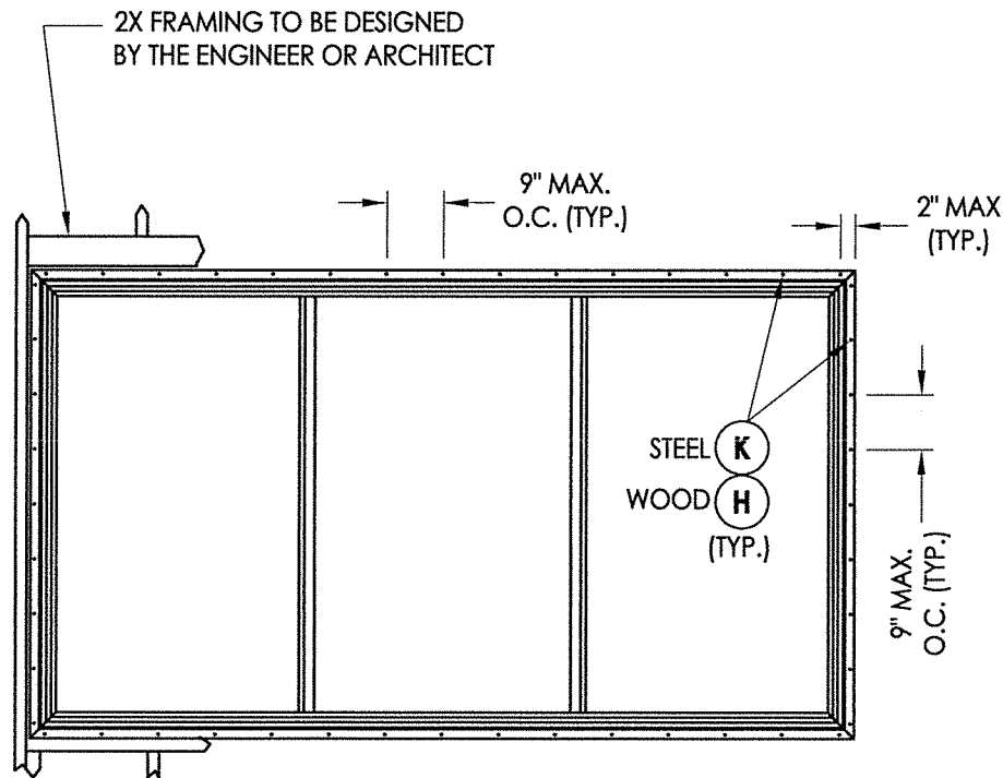
FRAME ANCHORING STUD CONSTRUCTION
