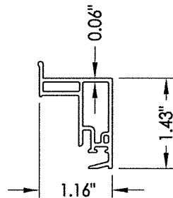
LOCK STILE
