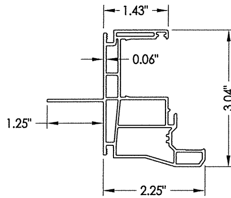
1 FRAME
