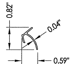
9 SCREEN CLIP
