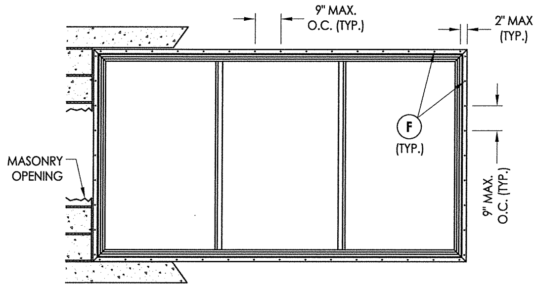
FRAME ANCHORING MASONRY CONSTRUCTION
