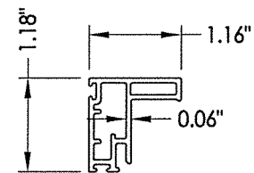
2 SASH STILE/RAIL
