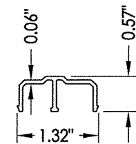
11 ROLLER TRACK
