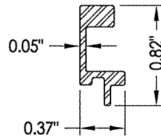
14 SASH STILE REINFORCEMENT
