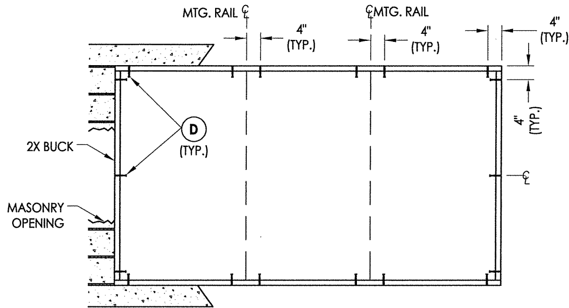
BUCK ANCHORING
