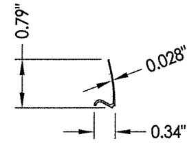
7 GLAZING BEAD
